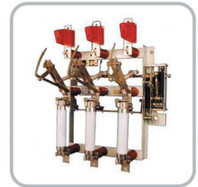
Load Break Switch
